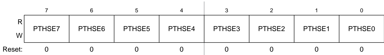
Figure 6-47. Slew Rate Enable for Port H Register (PTHSE)
