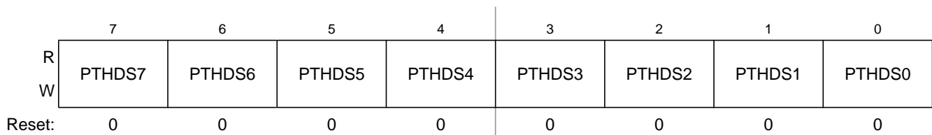
Figure 6-48. Drive Strength Selection for Port H Register (PTHDS)
