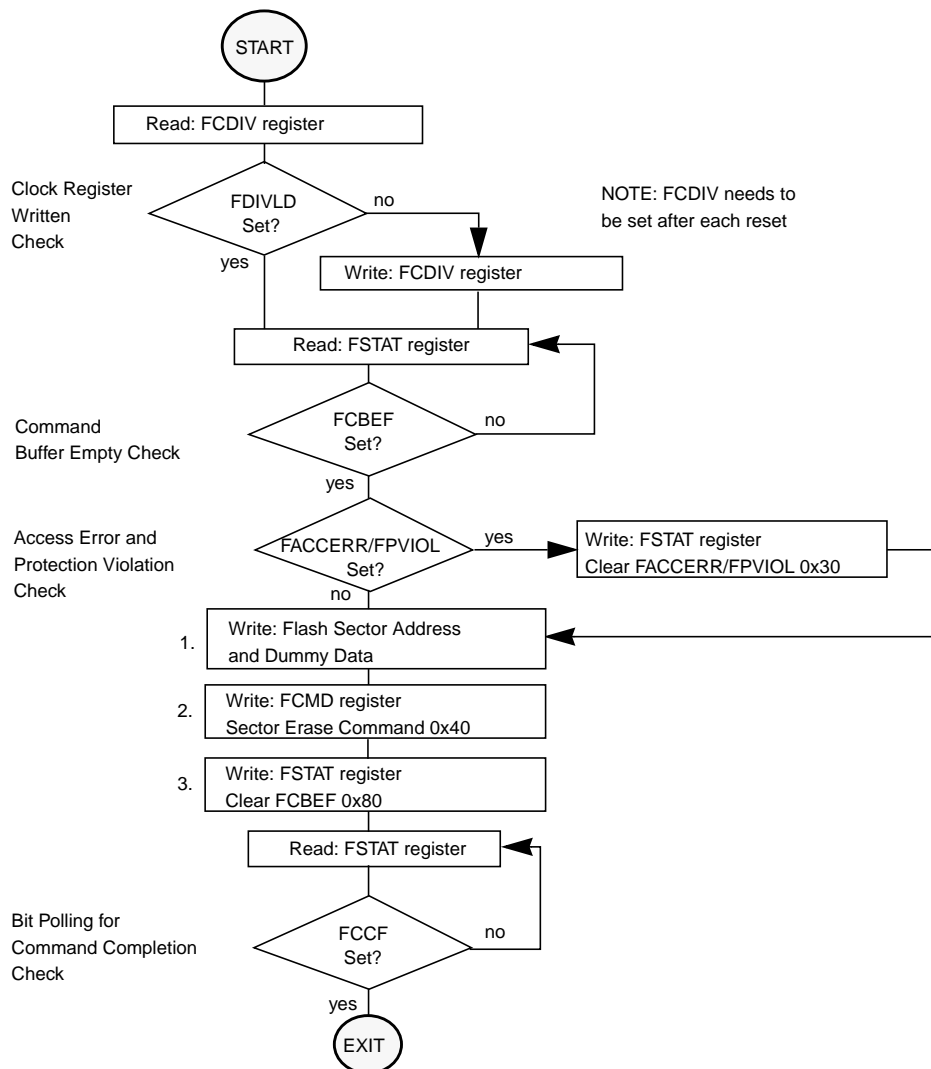
Figure 4-19. Example Sector Erase Command Flow
